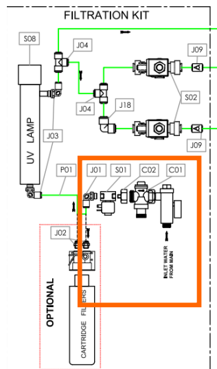
OLD HYDRAULIC DIAGRAM
